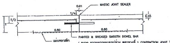
CONSTRUCTION JOINT
