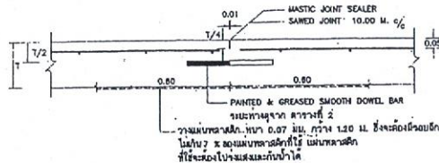
CONTRACTION JOINT
